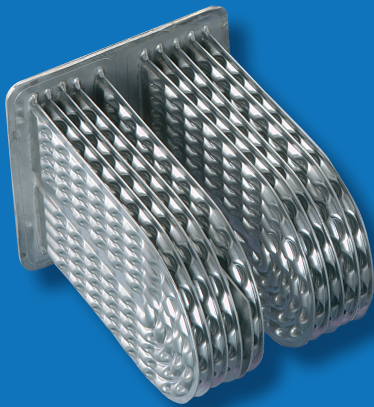
U-Plate Heat Exchanger
